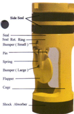
FlapperType
